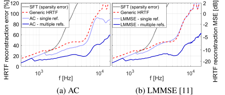
Fig. 2. HRTF reconstruction error using different approximation techniques
