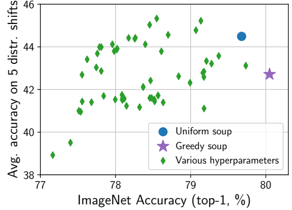
Figure E.2: Fine-tuning on ImageNet, using a ViT-B/32 [30] pre-trained on ImageNet-22k [23].
