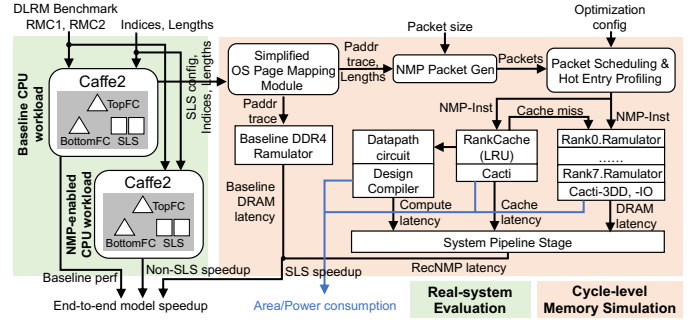
Fig. 13. RecNMP experimental methodology.
