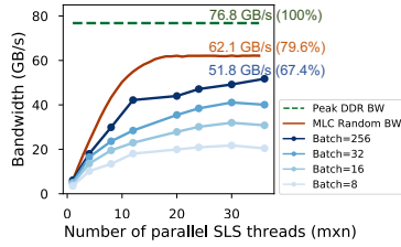
Fig. 5. Roofline of multi-threaded RMC1-large, RMC2-large sweeping batch size (1-256). Darker threads and batch sizes. color indicates larger batch.
