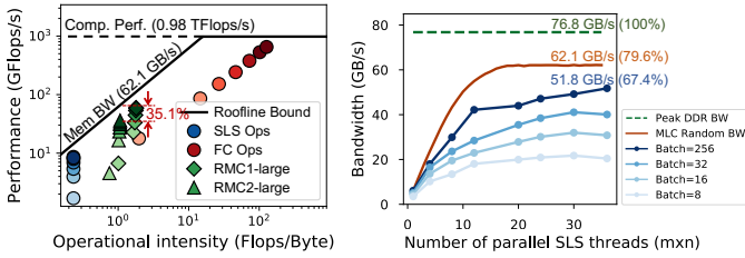
Fig. 5. Roofline of multi-threaded RMC1-large, RMC2-large sweeping batch size (1-256). Darker threads and batch sizes. color indicates larger batch.
