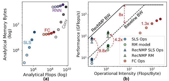
Fig. 1. (a) Compute and memory footprint of common deep learning operators, sweeping batch size; (b) Roofline lifting effect and the operator-level (FC, SLS) and end-to-end model (RM) speedup enabled by RecNMP .
