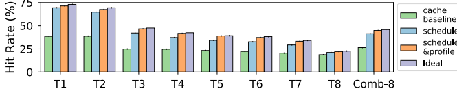
Fig. 11. NMP packet scheduling scheme that prioritizes batch of single table.
