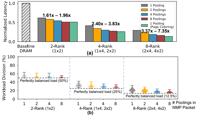
Fig. 14. (a) Normalized latency of RecNMP-base to the baseline DRAM with different memory configuration (DIMM x Rank) and NMP packet size; (b) Distribution of rank-level load imbalance for 2-, 4-, and 8-rank systems.
