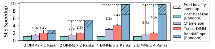
Fig. 16. Comparison between Host baseline, RecNMP-opt, TensorDIMM [81] and Chameleon [22] with both random and production traces
