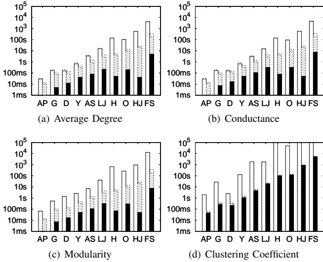
Fig. 7. Performance of Finding the Best k -Core Set
