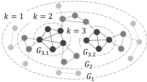
Fig. 1. Hierarchical Core Decomposition
