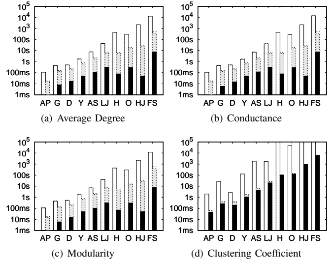
Fig. 8. Performance of Finding the Best Single k -Core
