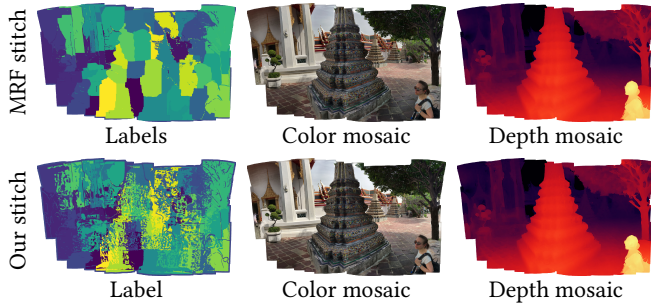
Fig. 5. Comparing stitching using MRF optimization (top row, runtime 3.25 minutes) vs. our algorithm (bottom row, runtime 0.5 seconds). While labels change more frequently in our solution, the color and depth mosaics are visually very similar to the MRF result.
