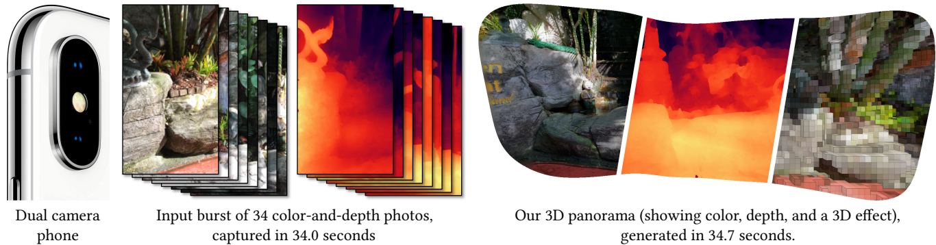
Fig. 1. Our work enables practical and casual 3D capture with regular dual camera cell phones. Left: A burst of input color-and-depth image pairs that we captured with a dual camera cell phone at a rate of one image per second. Right: 3D panorama generated with our algorithm in about the same time it took to capture. The geometry is highly detailed and enables viewing with binocular and motion parallax in VR, as well as applying 3D effects that interact with the scene, e.g., through occlusions (right).
