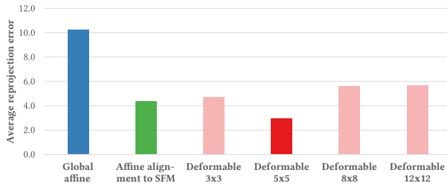
Fig. 8. Average reprojection error (Eq. 1, without the robust loss function ) for different alignment methods, as well as our deformable alignment with different grid sizes.
