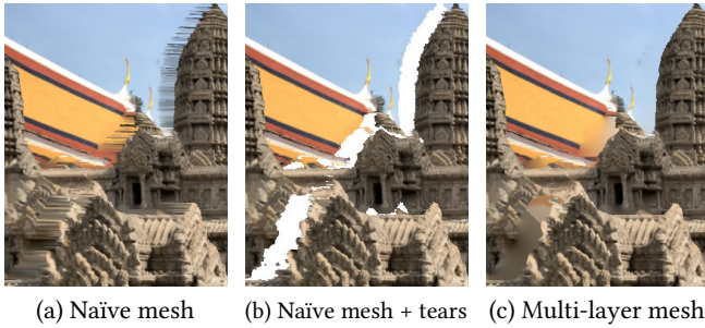
Fig. 6. (a) Naïvely meshing by connecting all vertices yield stretched triangles at depth edges. (b) Tearing the mesh avoids this, but reveals holes. (c) Our multi-layer meshes extend the back-side at depth edges smoothly into the occluded region and reveal in-painted colors and depths.
