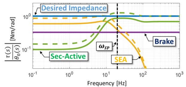
Figure 4. Frequency response of the desired and actuator torques normalized to the rendered impedance, in this case a nominal high stiffness of 77.5 kN/m. Hybrid approach is represented by solid lines and the active only is represented with dashed lines. Blue- desired response, orange - series elastic actuator, green- secondary active actuator, purple- passive actuator. \omega_{FP} filter cut-off for the frequency partitioning of the active actuators.
