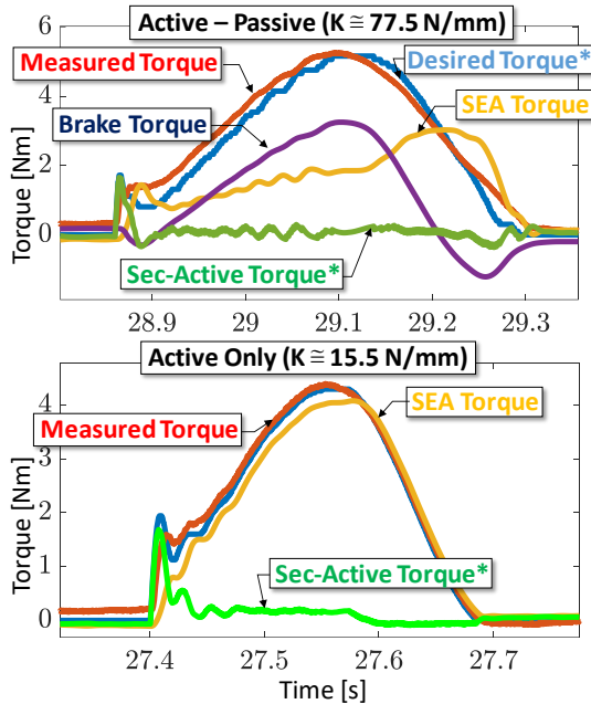
Figure 5. Time domain plot of the joint and the actuator torques while rendering a stiff virtual wall using the active-passive approach (top) and the active only approach (bottom). While the series elastic actuator and passive actuator torques are measured, the secondary actuator torque is the commanded torque. This can be more precisely measured by measuring the current on the secondary actuator.
