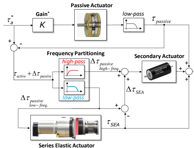
Figure 2. Block diagram representation of the Cascaded Passive-Active Only control approach. \tau_a^* is the desired actuator torque and \tau_a is the resulting actuator torque output from the three actuators. The gain* K is used to adjust the contribution of the passive actuator which is explained in detail in Section V. It is nominally set equal to 1. The measured passive actuator torque is low-pass filtered to remove sensor noise affecting the active command.
