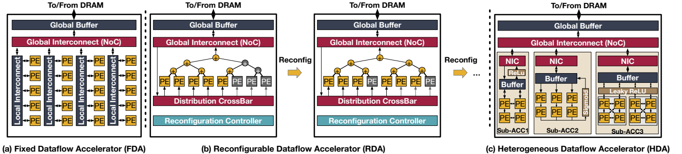
Fig. 3. Examples of fixed, reconfigurable, and heterogeneous dataflow accelerators.
