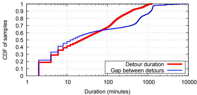
Figure 11: Distributions of EDGE FABRIC detour period lengths across (PoP, prefix) pairs and of time between detours.
