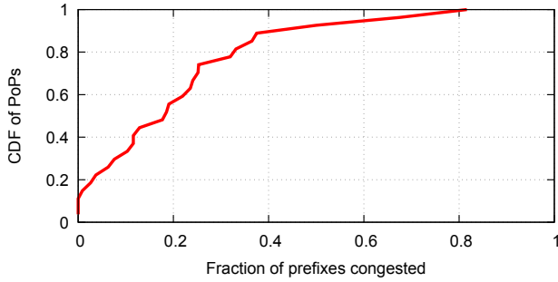
Figure 5: Distribution across PoPs of fraction of prefixes that would have experienced congestion had EDGE FABRIC not intervened.
