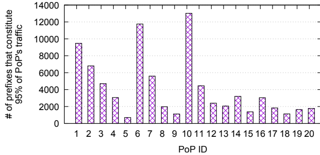
Figure 3: # of BGP prefixes to constitute 95% of PoP's traffic.
