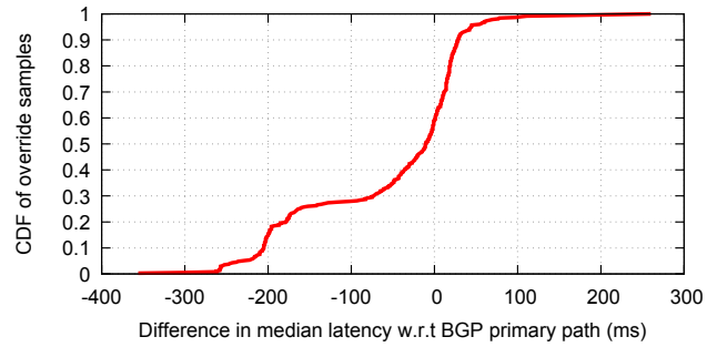
Figure 13: Performance difference between best paths chosen based on BGP policy and chosen based on alternate path measurements. Graph depicts latency-selected path minus policy-selected path, and so a negative value indicates that EDGE FABRIC’s override achieved better performance (lower latency).
