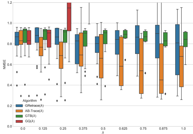
Figure 4. Comparison of empirical performance of GQ( \lambda ), AB-TRACE( \lambda ), GRETRACE( \lambda ) and GTB( \lambda ) on an off-policy evaluation task in Mountain Car domain. Each box plot shows the distribution of the NMSE achieved by each algorithm after 2000 episodes for different values of \lambda . NMSE distributions are computed over all the possible combinations of step-size values (\alpha_k, \eta_k) \in [0.001, 0.005, 0.01, 0.05, 0.1]^2 .
