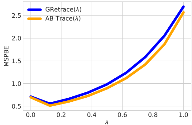
Figure 6. Comparison between the best empirical MSPBE obtained by each algorithm for different values of \lambda . Only GRETRACE( \lambda ) and AB-TRACE( \lambda ) are showed here because the other algorithms do not have the same operators and hence not the same MSPBE. Note that MSPBEs depend on \lambda . Thus, MSPBEs are not directly comparable across different values of \lambda . Both GRETRACE( \lambda ) and AB-TRACE( \lambda ) have very similar performances. AB-TRACE( \lambda ) performs slightly better.
