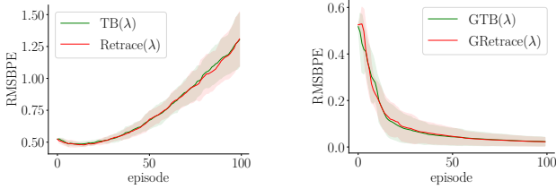
Figure 3. In the 2-states counterexample of section 3 showing that the gradient-based TB and RETRACE converge while TB and RETRACE diverge.
