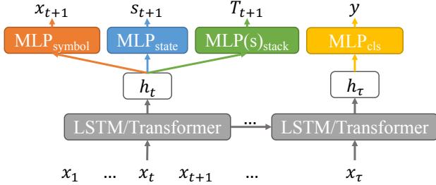
Figure 3: Oracle training.
