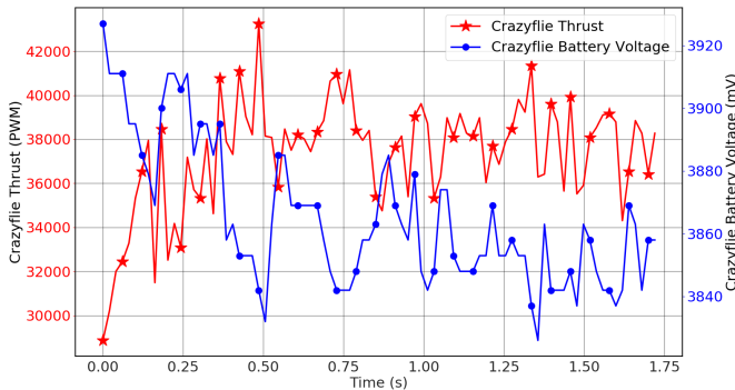
Fig. 11: The logged battery voltage and mean PWM of the 4 motors across a flight. There is a clear inverse relationship between the logged battery voltage and the current thrust.
