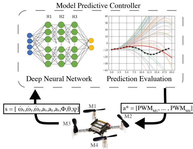
Fig. 1: The model predictive control loop used to stabilize the Crazyflie. Using deep model-based reinforcement learning, the quadrotor reaches stable hovering with only 10,000 trained datapoints – equivalent to 3 minutes of flight.
