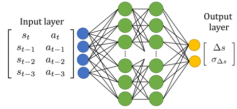
Fig. 3: The NN dynamics model predicts the mean and variance of the change in state given the past 4 state-action pairs. We use 2 hidden layers of width 250 neurons.
