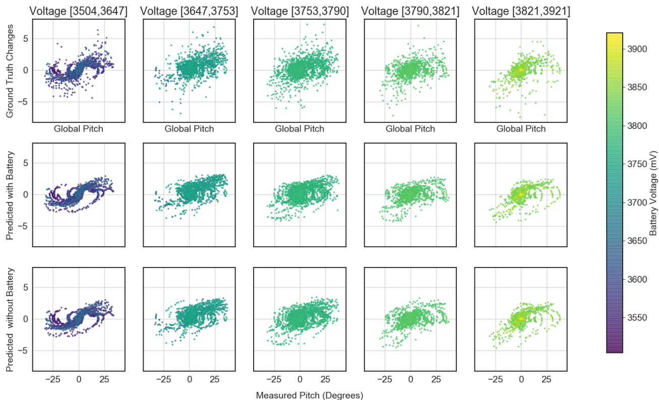
Fig. 9: Demonstration of the effect of battery voltage on state predictions. The top row is the ground truth one step pitch changes, the middle is the predictions through a model trained with battery voltage included in the state, and the bottom is predictions without battery voltage included in the state. Both of the predictions show tighter grouping from the variance term on the probabilistic loss function, but there is an extremely low difference between the predictions with and the predictions without battery. The lack of difference in predictions indicates the battery voltage is latent to other variables passed into the network.
