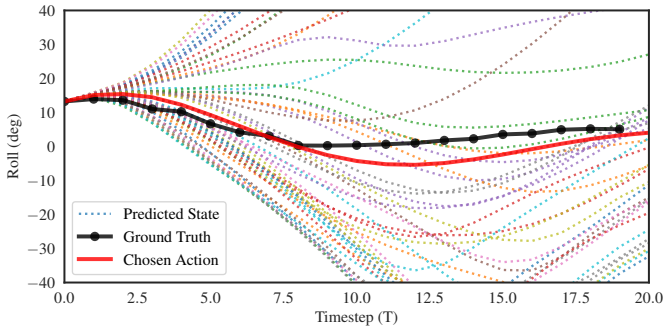
Fig. 4: Predicted states for N = 50 candidate actions with the chosen “best action” highlighted in red. The predicted state evolution is expected to diverge from the ground truth for future t because actions are re-planned at every step.
