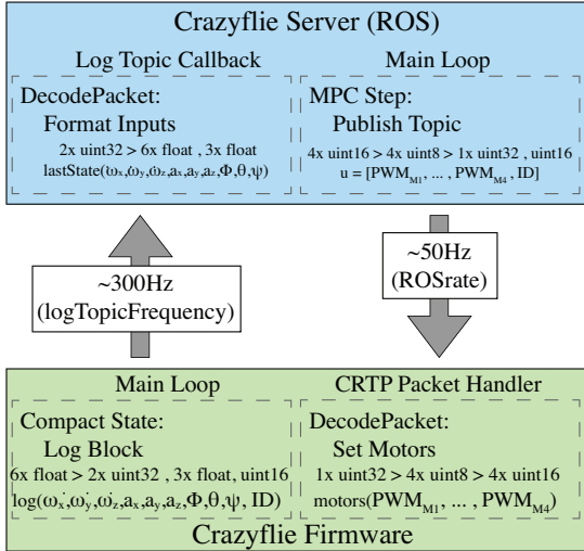
Fig. 2: The ROS computer passes control signals and state data between the MPC node and the Crazyflie ROS server. The Crazyflie ROS server packages Tx PWM values to send and unpacks Rx compressed log data from the robot.
