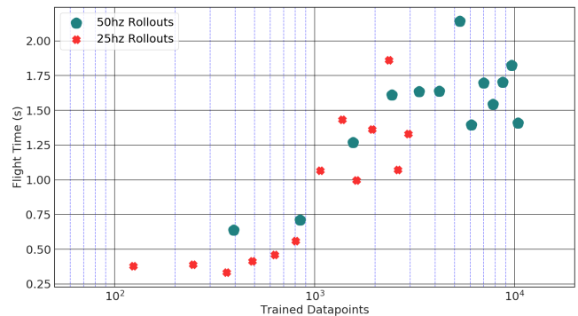
Fig. 12: Mean flight time of each rollout plotted verses the logarithm of the number of available points at train time for each model. The higher control frequency allows the controller to learn faster on wall time, but the plot indicates that there is not a notable difference between control ability when the number of trained points are equal. There is a continuing upward trend of flight time verses training points, but it is difficult to obtain more data in experiment.
