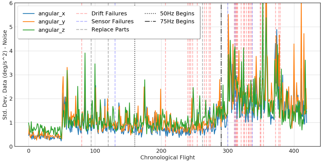
Fig. 10: The sensor noise on the 3 angular accelerations measured by the gyroscope of the MPU9250 of the Crazyflie before the robot takes off. The black vertical lines separate the rollouts at 25 Hz, 50 Hz and 75 Hz from left to right. The vertical lines indicate changes in hardware and collisions that would change the dynamics or state of the robot. The sensors clearly are subject to increasing noise over lifespan.
