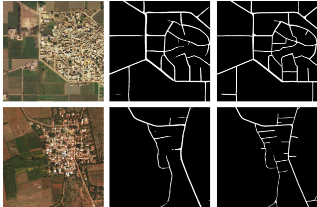
Figure 4: Example results of our road extraction method with an IoU score of 0.545, with satellite image (left), extracted road mask (middle), and the ground truth (right).
