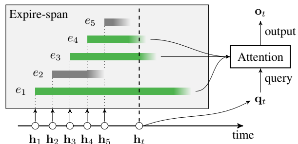
Figure 1. Expire-Span. For every memory h_i , we compute an EXPIRE-SPAN e_i that determines how long it should stay in memory. Here, memories h_2 , h_5 are already expired at time t , so the query q_t can only access \{h_1, h_3, h_4\} in self-attention.
