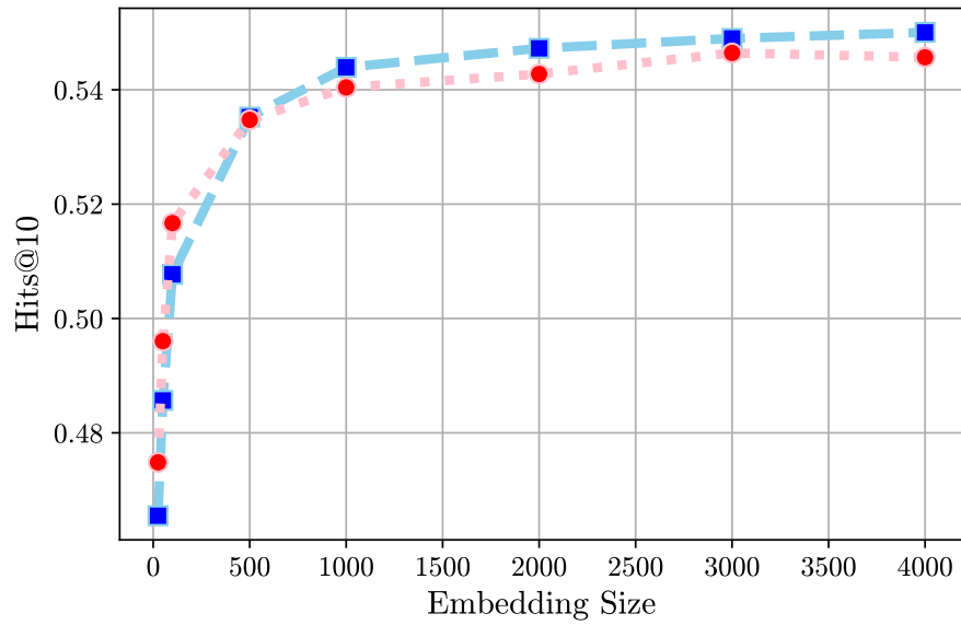
Figure 7: Hits@10 versus Rank for CP on FB15k-237.
