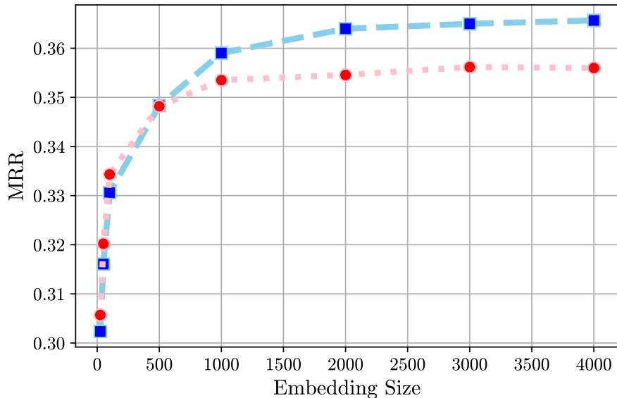
Figure 5: MRR versus Rank for CP on FB15k-237.
