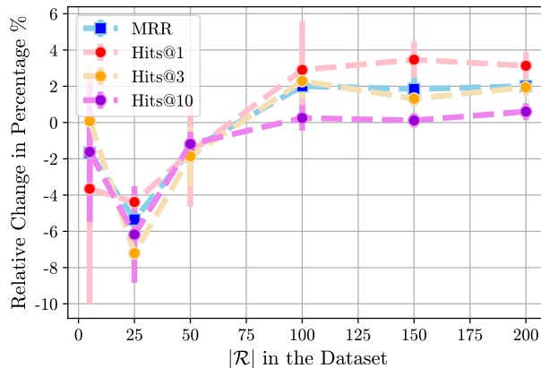
Figure 1: Relative changes between ComplEx trained with and w/o Relation Prediction on datasets with varying numbers of predicates |\mathcal{R}| . We experimented with 3 random seeds. Larger bars mean more variance. Relative changes were computed with (m_+ - m_-)/m_- , where m_+ and m_- denote the metric values with and w/o relation prediction. A clear downward trend can be observed for datasets with |\mathcal{R}| < 50 while 2% – 4% clear increase in MRR, Hits@1, and Hits@3 are shown where |\mathcal{R}| > 50 .
