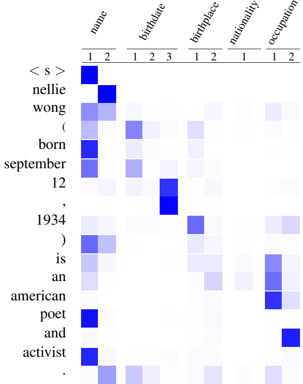
Figure 4: Visualization of attention scores for Nellie Wong’s Wikipedia infobox. Each row represents the probability distribution over (field, position) pairs given the previous words (i.e. the words heading the preceding rows as well as the current row). Darker colors depict higher probabilities.
