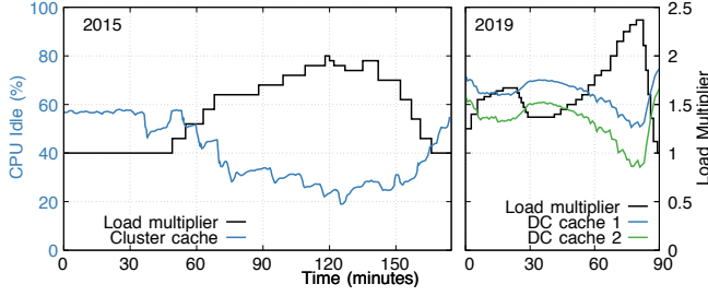
Figure 14. Sensitivity analysis for the same services in 2015 and 2019, respectively. The analysis in 2015 takes almost twice as long as the one in 2019. The impact on the backend systems is visible. Specifically, in 2015, there are icicles at the beginning of each step—the introduction of cold traffic leads to cache misses and results in CPU spikes at the backends.
