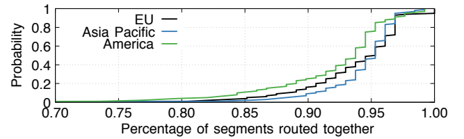
Figure 11. The probability of the percentage of segments routed together (to the same data centers) at three different edge nodes over the course of a day. Taiji routes 95%+ of the segments together for 80% of the time (the other segments are further split up and routed at the bucket granularity).
