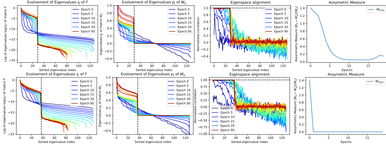
Figure 2. Training BYOL in STL-10 for 100 epochs with EMA. Top row : No symmetric regularization imposed on W_p , Bottom row : symmetric regularization on W_p . From left to right: (1) Evolution of eigenvalues for F . Since F is PSD and its eigenvalue s_j varies across scales, we plot \log(s_j) . We could see some eigenvalues are growing while others are shrinking to zero over training. (2) Similar “step-function” behaviors for the predictor W_p . Its negative eigenvalues shrinks towards zero and leading eigenvalues becomes larger. (3) The eigenspace of F and W_p gradually align with each other (Theorem 3). For each eigenvector u_j of F , we compute cosine angle (normalized correlation) between u_j and W_p u_j to measure alignment. (4) W_p gradually becomes symmetric and PSD during training.
