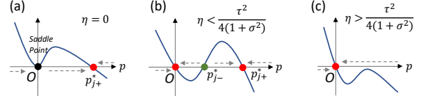
Figure 4. Fixed point of \dot{p}_j = p_j(p_j - p_{j-}^*)(p_j - p_{j+}^*) . Stable fixed points are in red, unstable in green and saddle in black. When the weight decay \eta = 0 , the trivial solution p_j = 0 is a saddle. When \eta > 0 , the trivial solution becomes stable near to the origin and initial p_j needs to be large enough to converge to the stable non-collapsed solution p_{j+}^* .
