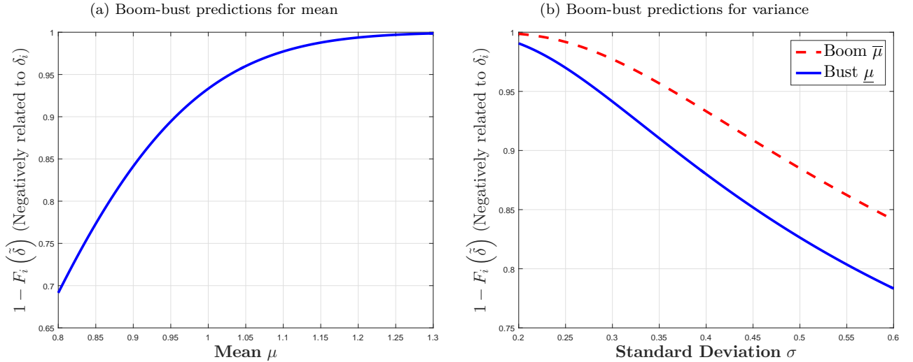
Figure 2: Housing-as-consumption predictions
