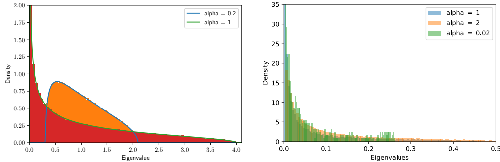
Figure 10: Spectrum of the logistic regression loss with tanh unit: when data has a single Gaussian blob (left), when data has two Gaussian blobs (right). In the latter case, the spectrum has outlier eigenvalues at 454.4, 819.5, and 92.7 for alpha = 1, 2, 0.02 , respectively.
