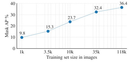
(c) Low-shot detection is an open problem: training Mask R-CNN on 1k images decreases COCO \text{val}_{2017} mask AP from 36% to 10%.
