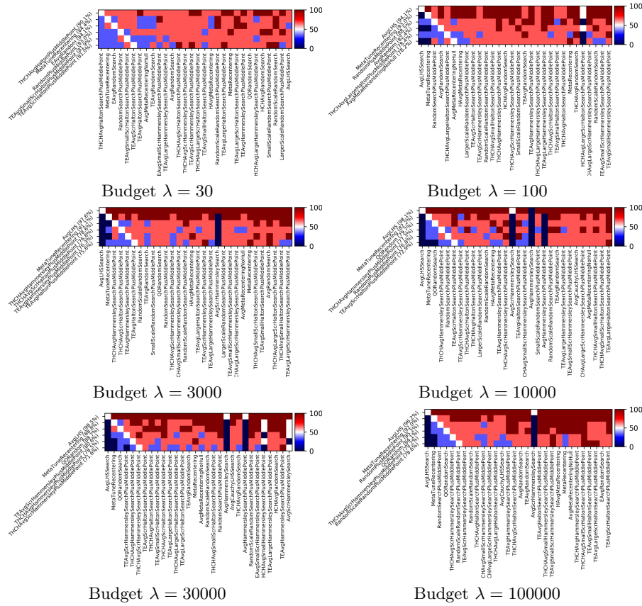
Fig. 5. Results on the sphere function, per budget. Results are averaged over dimension 20, 200, 2000. Our method MetaTuneRecentering performs among the best in all cases. LHS is excellent on this very simple setting, namely the sphere function.
