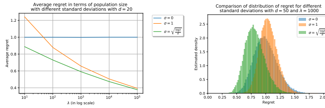
Fig. 2. Comparison of methods: without rescaling ( \sigma = 1 ), middle point sampling ( \sigma = 0 ), and our rescaling method ( \sigma = \sqrt{\frac{\log \lambda}{d}} ). Each mean has been estimated from 10^5 samples. (On left) Average regret, normalized by d , on the sphere function for diverse population sizes \lambda at fixed dimension d = 20 . The gain of rescaling decreases as \lambda increases. (On right) Distribution of the regret for the strategies on the 50d -sphere function for \lambda = 1000 .
