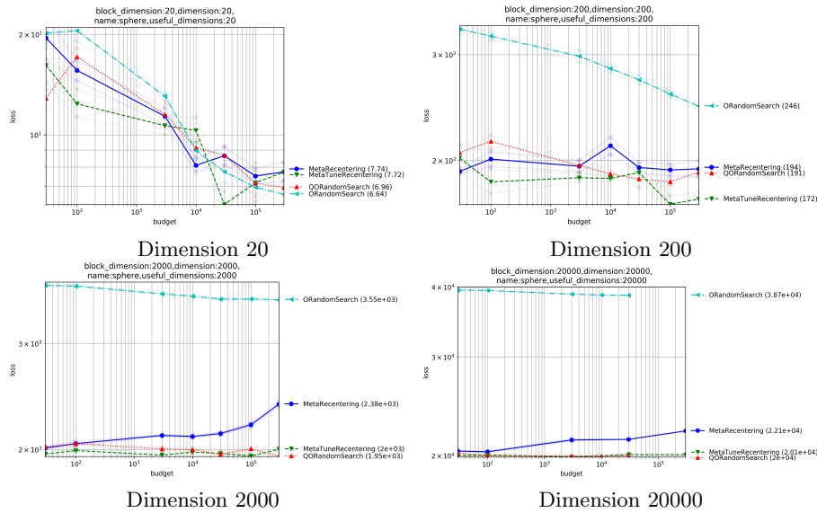
Fig. 7. Same context as Fig. 6, with x -axis = budget and y -axis = average simple regret. We see the failure of MetaRecentering as budget goes to infinity: the budget has an impact on \sigma which becomes worse, hence worse overall performance. We note that quasi-opposite sampling can perform decently in a wide range of values. Opposite Sampling is not much better than random search in high-dimension. Our MetaTuneRecentering shows decent performance: in particular, simple regret decreases as \lambda \rightarrow \infty .
