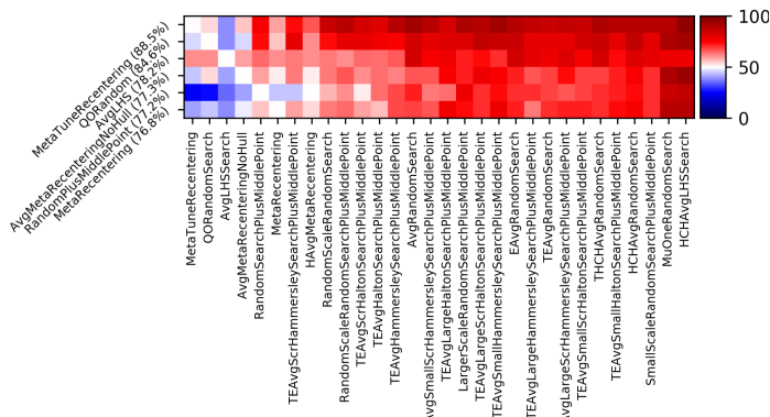
Fig. 3. Comparison of various one-shot optimization methods from the point of view of the simple regret. Reading guide in Sec. 4.2. Results are averaged over objective functions Cigar, Rastrigin, Sphere in dimension 20, 200, 2000, and budget 30, 100, 3000, 10000, 30000, 100000. MetaTuneRecentering performs best overall. Only the 30 best performing methods are displayed.
