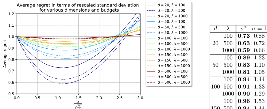
Fig. 1. Average regret, normalized by d , on the sphere function for various dimensions and budgets in terms of rescaled standard deviation. Each mean has been estimated from 100,000 samples. Table on the right: Average regret for \sigma^* = \sqrt{\log(\lambda)/d} and \sigma = 1 .
