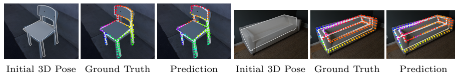
Fig. 6: Qualitative examples of our predicted geometric correspondence fields. Our predicted 2D displacement vectors are highly accurate. Best viewed in digital zoom .
