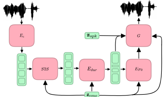
Figure 1: An illustration of the proposed system. The input signal is first encoded as a discrete sequence of content units ( E_c ). Next, a sequence to sequence ( S2S ) model is applied to translate between the sequences corresponding to different emotions. Then we predict the duration ( E_{dur} ) and F0 ( E_{F0} ) before feeding these signals to a vocoder ( G ). The last 4 components are conditioned by emotion ( z_{emo} ). We use pink to denote models and green to denote representations.
