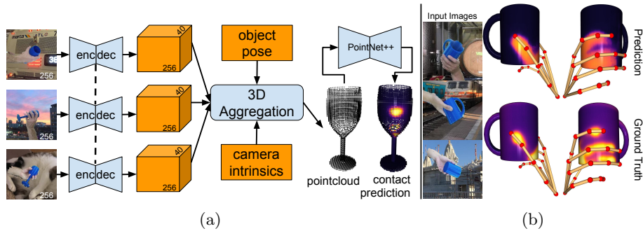
Fig. 11: (a) Image-based contact prediction architecture. (b) Contact prediction for mug (an unseen object) from RGB images, using networks trained with 3 views. Hand poses shown only for reference.
