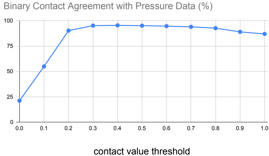
Fig. 12: Relation of contact value threshold to the binary contact agreement with pressure data from the Sensel Morph sensor. Agreement maximizes at the threshold value of 0.4.
