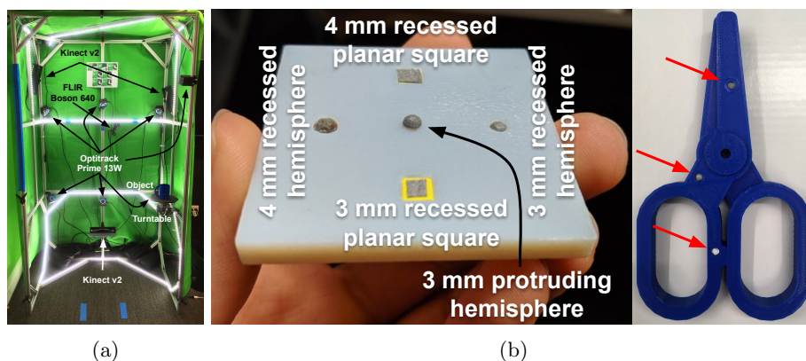
Fig. 3: (a) Our setup consists of 7 Optitrack Prime 13W tracking cameras, 3 Kinect v2 RGB-D cameras, a FLIR Boson 640 thermal camera, 3D printed objects, and a turntable. (b) Left : Different object tracking marker configurations we investigate. Right : 3D printed object with recessed 3 mm hemispherical markers (highlighted by red arrows) offer a good compromise between unobtrusiveness and tracking performance.
