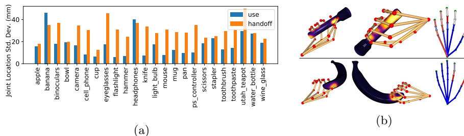
Fig. 8: (a) Per-object standard deviation in 3D joint locations, for ‘use’ and ‘hand-off’. ‘Hand-off’ grasps consistently exhibit more diversity than ‘use’ grasps. (b) A pair of grasps with similar hand pose but different contact characteristics. Hand contact feature color-coding is similar to Figure 5a.
