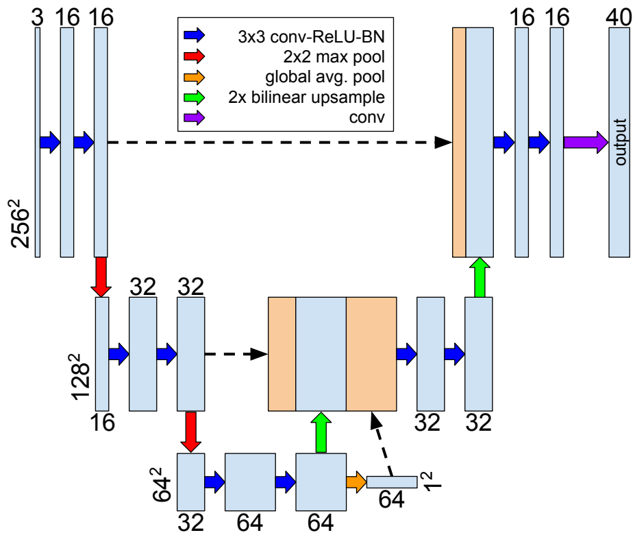
Fig. 15: Architecture for the image encoder-decoder (Figure 10 in main paper). Horizontal numbers indicate number of channels, and vertical numbers indicate spatial dimensions.
