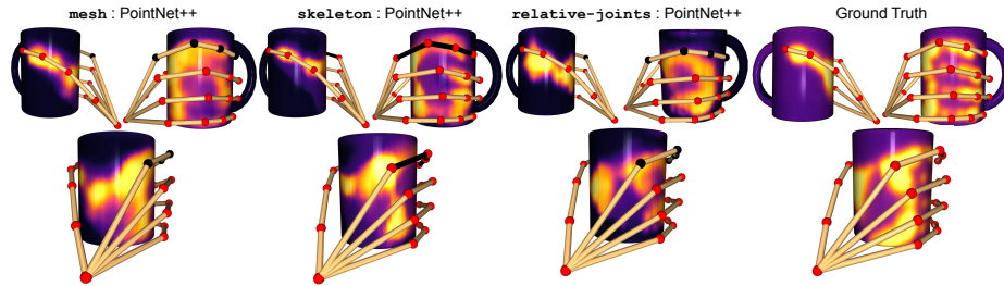
Fig. 10: Contact prediction for mug (an unseen object) from hand pose. All input features related to black line segments and joints were dropped (set to 0). Notice how the mesh- and skeleton- PointNet++ predictors is able to capture nuances of palm contact, thumb and finger shapes.
