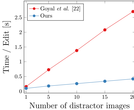
Fig. S8: Time analysis of multi-distractor setup.
