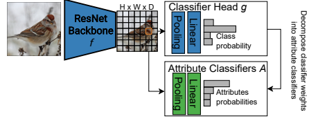
Fig. 6: Attribute-based decomposition.
