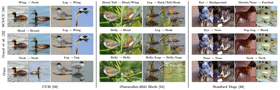
Fig. 3: State-of-the-art comparison of counterfactual explanations (Single Edit - VGG-16). Part labels are included only for better visualization. Image credit: [1]
