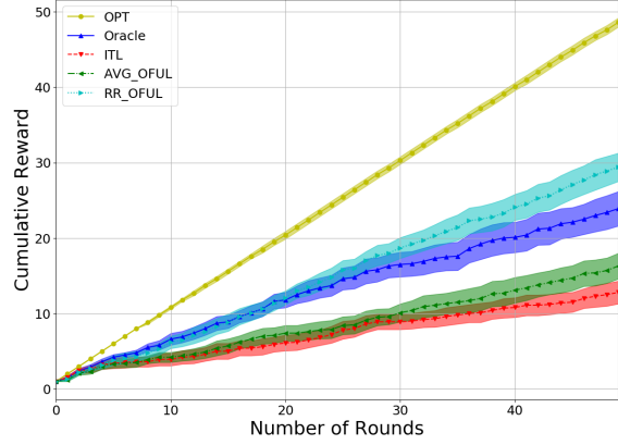
Figure 1. Cumulative reward measured after N = 10 tasks and averaged over 10 independent test tasks, with \lambda = 1 .
