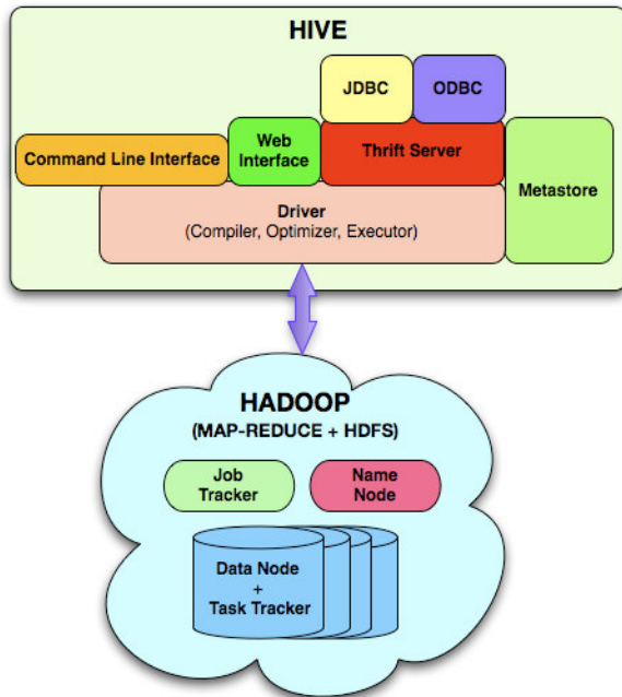
Figure 2: Hive System Architecture
