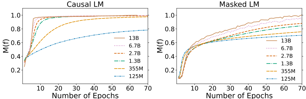
Figure 11: Proportion of training data memorized M(f) over training, for causal (Left) and masked (Right) language modeling on WIKITEXT103. The x -axis describes the number of epochs, and y -axis denotes M(f) as defined in § 3. Generally, we see that larger models memorize training data faster.
