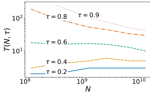
Figure 2: T(N, \tau) as a function of N (shown on log-log scale), for various values of \tau in masked language modeling on WIKITEXT103. We show that larger models initially memorize training data slower, but reach high proportions of training data memorization faster.
