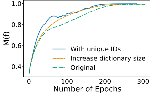
Figure 6: The impact of adding unique identifiers to training examples on memorization M(f) training dynamics for causal language modeling (125M) on WIKITEXT103. The green line is the original 125M model. The orange line is the model after adding unique identifiers to the dictionary (which increases model size). The blue line prepends these unique identifiers for each training example. Note that adding unique identifiers leads to faster memorization of training data.
