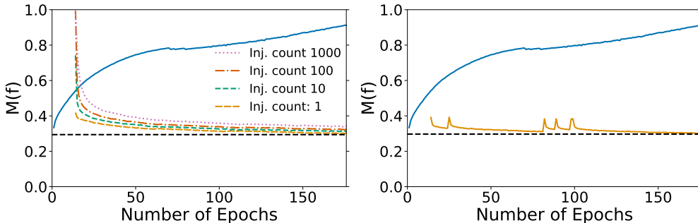
Figure 10: Effect of repeated injection (Left) and spaced repetition (Right) on special batch memorization. Results are for causal language modeling (125M) on WIKITEXT103. The solid upper curve represents the training set memorization. We show that repeated injection increases the forgetting baseline, whereas spaced repetition has minimal effect.
