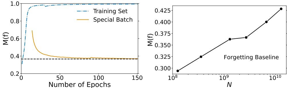
Figure 8: Left: forgetting curve for causal language modeling (2.7B) on WIKITEXT103. The dashed horizontal line indicates the lowest proportion of special batch data memorized throughout training, i.e., the forgetting baseline. Right: forgetting baseline as a function of model size N (plotted on log scale). We show that as model scale increases, the forgetting baseline value increases.
