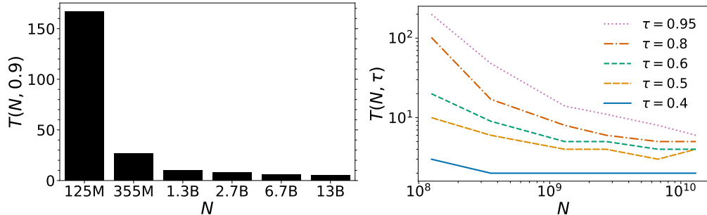
Figure 1: We show T(N, \tau) , which is the number of times a language model needs to see each training example before memorizing \tau fraction of the training data, as a function of model size N . Result are for causal language modeling on WIKITEXT103, right plot is on log-log scale. Note that generally larger models memorize faster, regardless of \tau .
