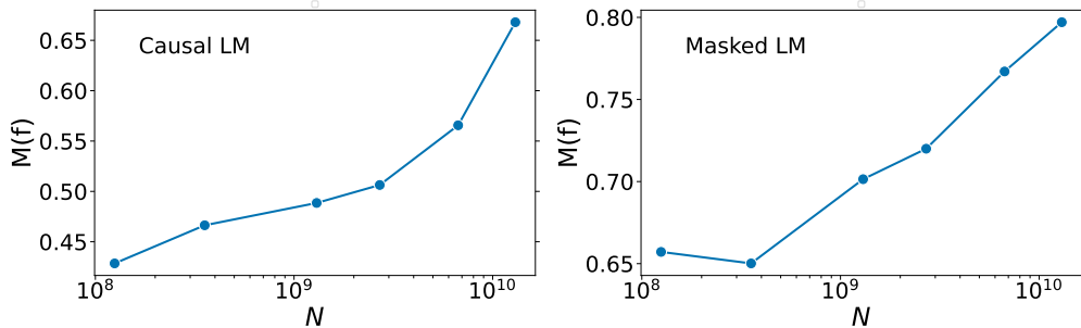
Figure 4: Proportion of training data memorized M(f) before overfitting, as a function of model size N (plotted on a log scale). Results are for causal (left) and masked (right) language modeling on WIKITEXT103. Note that larger models memorize more before overfitting.
