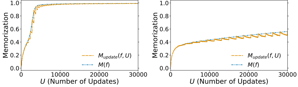
Figure 13: We show training data memorization evaluated at the end of an epoch M(f) , and at the end of each gradient descent update M_{update}(f, U) , over training. Results shown are for causal language modeling on WIKITEXT103 dataset for 13B (Left) and 125M (Right) model sizes. We note that M_{update}(f, U) closely tracks M(f) throughout training.
