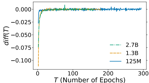
Figure 15: Exploring the sequential difference in proportion of training data memorized M(f) on the special batch over training. The x -axis denotes the number of epochs (i.e. T ) and the y -axis denotes the sequential difference in M(f) from the (T - 1) 'th epoch to the T 'th epoch (i.e. \text{diff}(T) ). Results shown are for causal language modeling on WIKITEXT103. We show that sequential difference in memorization exponentially approaches 0.
