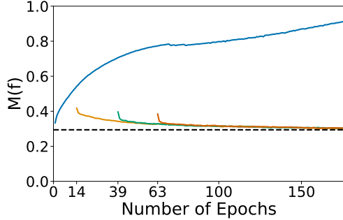
Figure 9: We empirically show that the forgetting baseline does not depend on data batch ordering. We inject the special batch into the training set at the 14th, 39th, and 63rd epochs, and evaluate proportion of special batch data memorized as we continue training. Results are for causal language modeling (125M) on WIKITEXT103.
