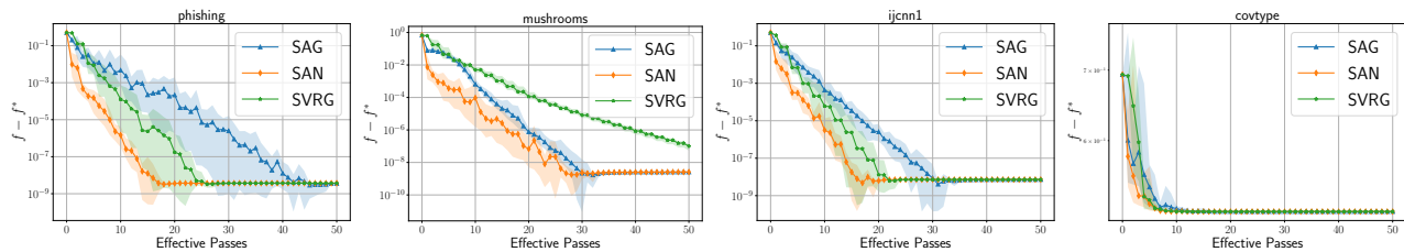
Figure 3: Function sub-optimality of logistic regression with L2 regularization.
