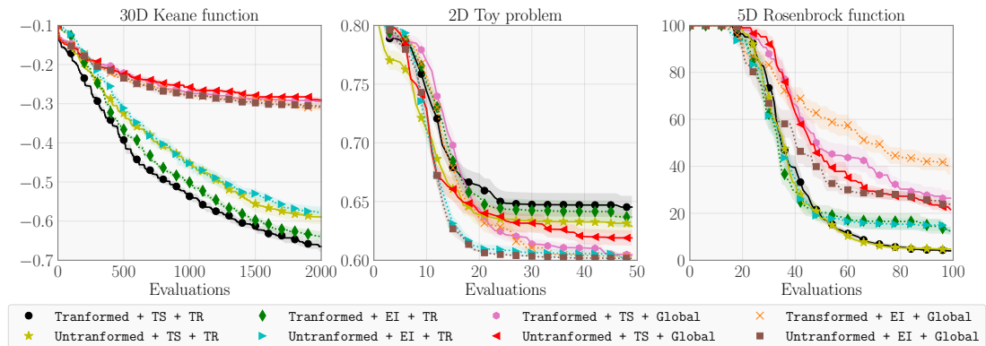
Figure 5: We investigate the effect of using the robust transformation, different acquisition functions (TS/EI), and using a trust region (TR). (Left) 30D Keane function with 2 black-box constraints. (Middle) 2D Toy problem with 2 black-box constraints of Hernández-Lobato et al. [2016]. (Right) 5D Rosenbrock function with 2 poorly scaled black-box constraints.
