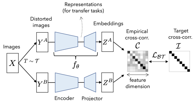
Figure 1. BARLOW TWINS’s objective function measures the cross-correlation matrix between the output features of two identical networks fed with distorted versions of a batch of samples, and tries to make this matrix close to the identity. This causes the embedding vectors of distorted versions of a sample to be similar, while minimizing the redundancy between the components of these vectors. BARLOW TWINS is competitive with state-of-the-art methods for self-supervised learning while being conceptually simpler, naturally avoiding trivial constant (i.e. collapsed) embeddings, and being robust to the training batch size.
