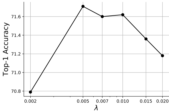
Figure 5. Sensitivity of BARLOW TWINS to the hyperparameter \lambda
