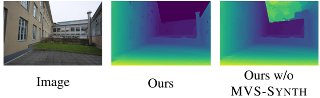
Figure 10. Comparisons between networks trained with and without the MVS-SYNTH dataset. Without MVS-SYNTH dataset, the network has difficulty in handling regions such as the sky because real-world datasets do not cover these regions.
